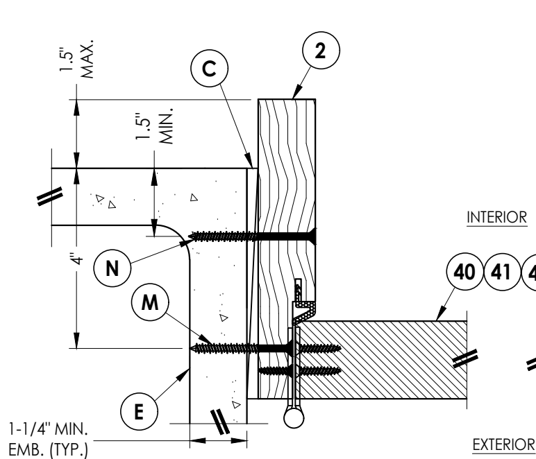
5/6 HORIZONTAL CROSS SECTION Shown Direct to Masonry Outswing only w/ 6-9/16" jamb
